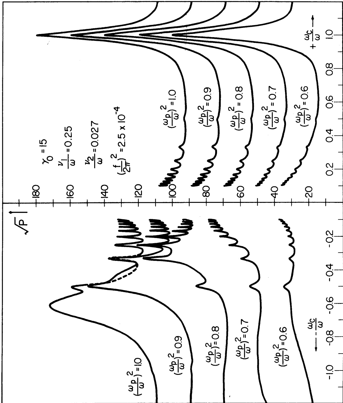
Fig. 2 Typical theoretical emission spectra in the neighborhood of the electron cyclotron frequency
