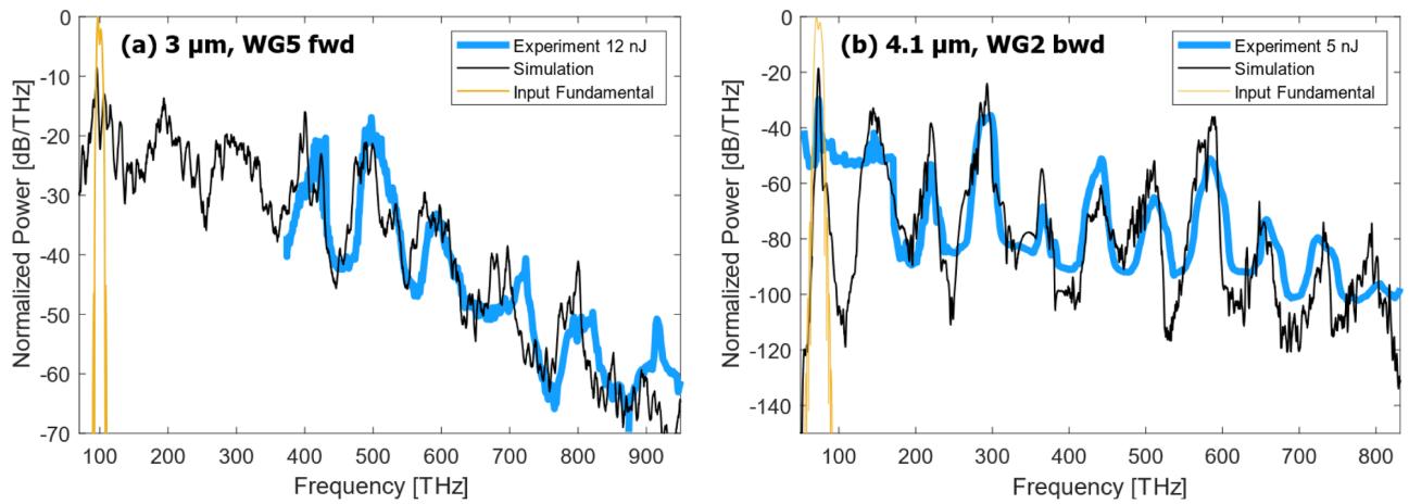
Fig. 5. (a) Overlay of simulated output spectrum (thin black line) and input pump spectrum (thin yellow line) having \mathcal{R} = L_{GVM}/L_{NL}^{(2)} = 5.74 with experimental data (thick blue line) for 3 \mu\text{m} , 12 nJ pumping in Waveguide 5, forward. (b) Idem for 4.1 \mu\text{m} pumping in Waveguide 2, backward with \mathcal{R} = 1.57 and 5 nJ experimental pulse energy. Experimental data in (b) is from the study first reported in [26].
