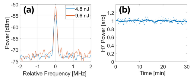
Fig. 4. (a) Heterodyne beat notes (100 kHz resolution bandwidth) between the sixth harmonic from the waveguide and second harmonic of the Yb: fiber pump comb used in the OPA, verifying the harmonic coherence. (b) Measured power in a 0.7 nm bandwidth at the seventh harmonic (428 nm) over a 30 min duration, highlighting the long-term stability of this experimental setup. Dotted points represent 10 s measurement bins, and the solid line is their smoothed average.
