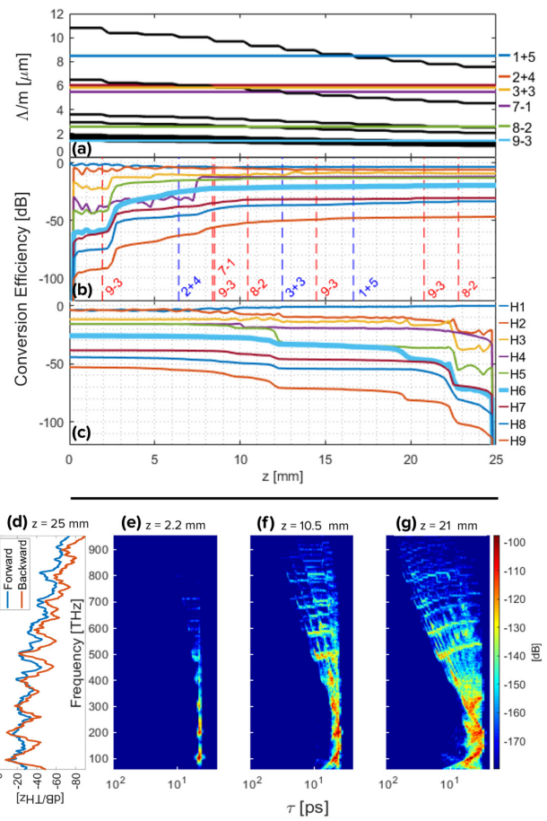
Fig. 7. (a) Higher-order poling periods of Waveguide 5 (black) intersected by the phase-matching solutions (horizontal colored) of SFG/DFG processes generating the sixth harmonic of 3\ \mu\text{m} . (b), (c) Harmonic evolution throughout propagation in the forward and backward pumping direction for the same \mathcal{R} as Fig. 5(a), overlaid with the phase-matched locations of SFG (blue dashed) and DFG (red dashed) processes generating H6 (thick blue line). While the QPM direction indeed alters each harmonic's growth history, ultimately their conversion efficiencies are similar, further highlighted in (d) by the forward (blue) and backward (orange) output spectra. (e)–(g) Time-frequency spectrograms corresponding to (b) at three waveguide locations, showing the dispersion of generated harmonics and their temporal overlap throughout propagation.
