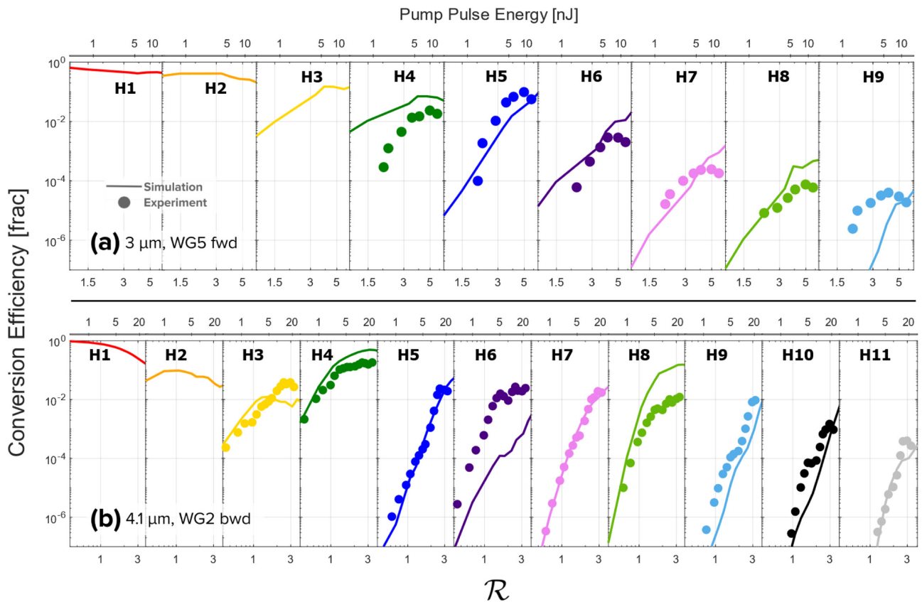
Fig. 6. Harmonic power scaling in terms of both the simulated \mathcal{R} \equiv L_{GVM}/L_{NL}^{(2)} (bottom axes, lines) and experimental pump-pulse energy (top axes, dots) for (a) 3 \mu\text{m} , Waveguide 5, forward, and for (b) 4.1 \mu\text{m} , Waveguide 2, backward, with 4.1 \mu\text{m} experimental data from [26]. Both experiments show saturation of harmonics at \mathcal{R} \approx 3 .
