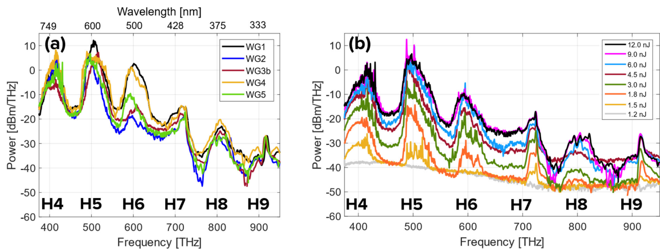
Fig. 2. (a) Comparison of measured spectra for all five waveguides at 12 nJ pumping. Designation “b” for WG3 indicates that harmonics were measured in the backward (increasing poling period) pumping direction. Qualitatively similar spectra are observed from each of the waveguides. (b) Measured spectra at various pump pulse energies in Waveguide 5. The harmonics first appear at 1.5 nJ and saturate around 9 nJ.
