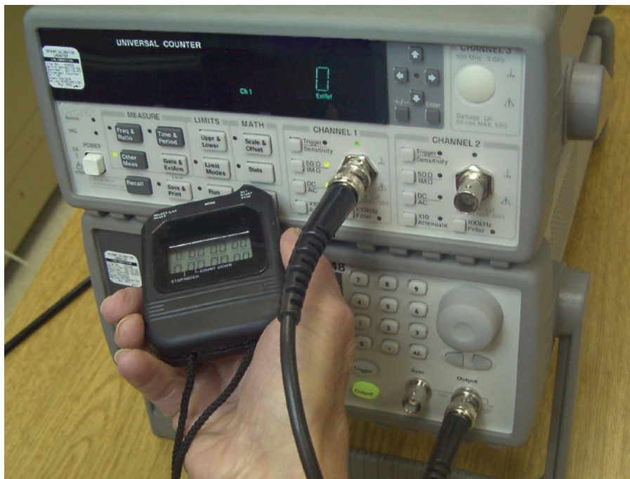
Figure 1. A stopwatch calibration that employs the totalize function of a universal counter (courtesy of Sandia National Laboratories).
