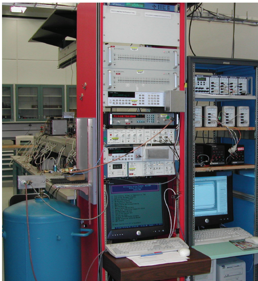
Figure 7. Josephson voltage standards require a high performance frequency reference (courtesy of Yi-hua Tang, NIST).
