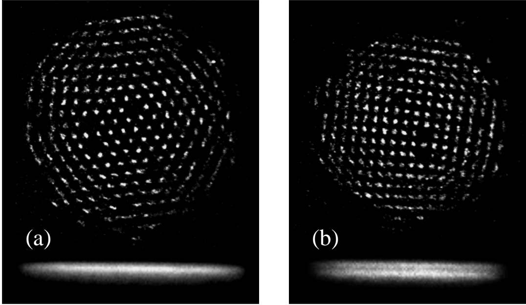
FIGURE 5. Strobed top-view images of a small ( N \sim 300 \text{Be}^+ ) ion plasma phase-locked with a rotating dipole field at (a) \omega_r = 2\pi \times 65.7 kHz and (b) 66.5 kHz. Below are unstrobed side-views showing the axial lattice planes. Heavier-mass ions are located outside the ^9\text{Be}^+ ions.
