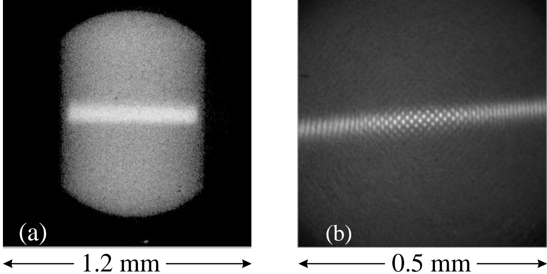
FIGURE 4. Real-space images of an N \sim 1.8 \times 10^5 ion plasma phase-locked with an oscillating dipole field at \omega_r = 2\pi \times 120 kHz. (a) Time-averaged side-view image showing the overall plasma shape. The bright line of fluorescence through the plasma center is due to a laser beam directed perpendicularly to \mathbf{B}_0 . The plasma shape is approximately spherical. The presence of heavier-mass ions, which centrifugally separate from the {}^9\text{Be}^+ ions, produces the straight vertical boundaries in the image. (b) Strobed top-view image, obtained simultaneously with (a), showing the presence of a bcc crystal in the plasma center. The distance scales in (a) and (b) are different as noted.
