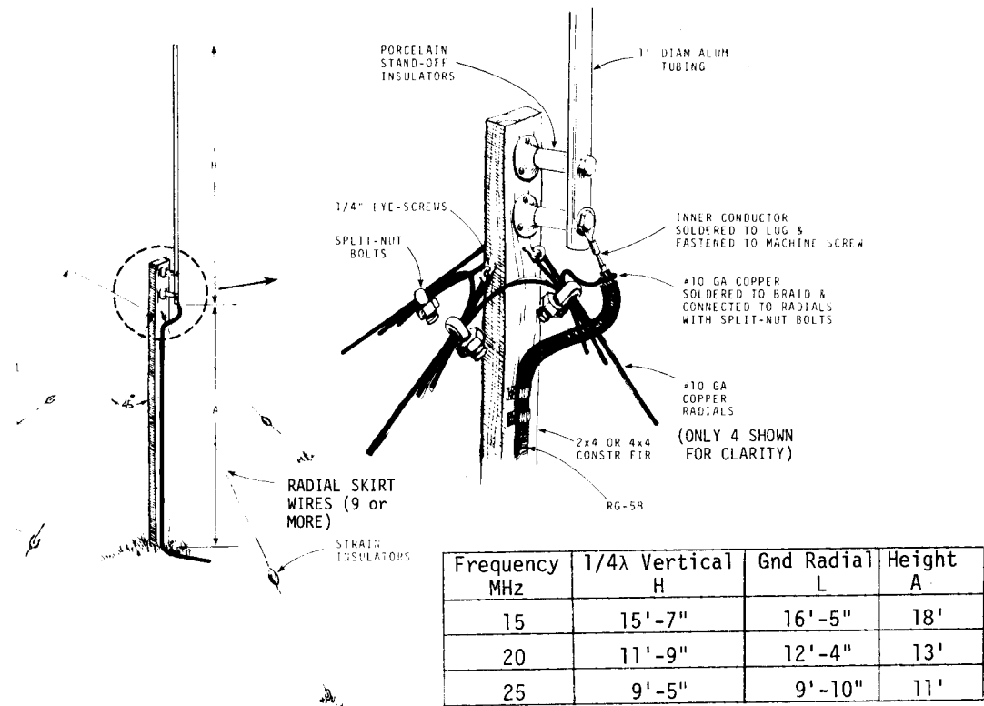
Figure 19. Modified half-wavelength vertical antenna for use at 15, 20, and 25 MHz.
