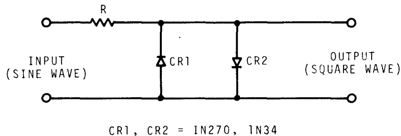
Figure 13. Diode clipping circuit to produce harmonics from a pure sine wave signal.
