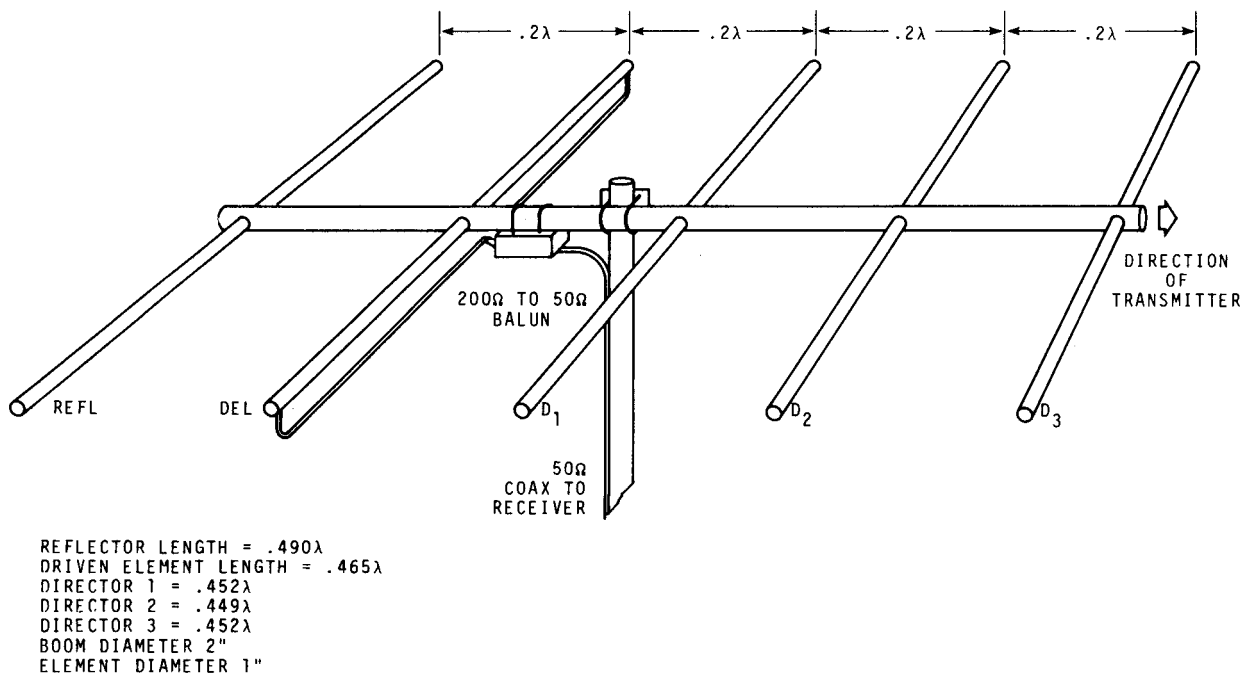
Figure 20. Typical Yagi antenna design
