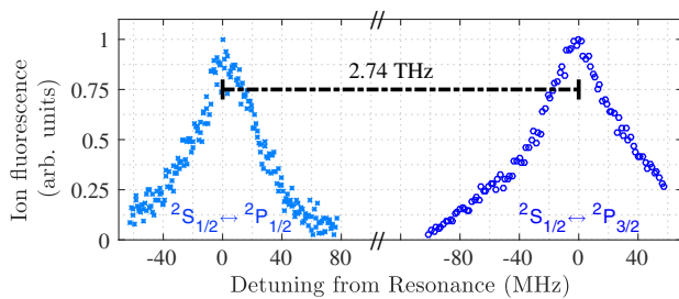
Fig. 6. Spectroscopy of the ^2S_{1/2} \leftrightarrow ^2P_{1/2} and ^2S_{1/2} \leftrightarrow ^2P_{3/2} transitions of a single trapped ^{25}\text{Mg}^+ ion. The zero detuning points of the transitions from the ^2S_{1/2} to the ^2P_{1/2} and ^2P_{3/2} levels are relative to 1069.34 and 1072.08 THz, respectively [35]. The fine-structure separation is approximately 2.74 THz. Each spectrum is independently normalized.
